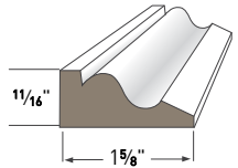
BAND MOULDING AZM-217 Length: 16'
