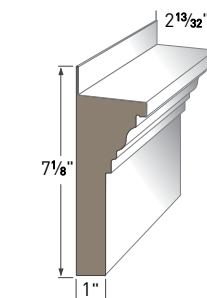
CROSSHEAD PEDIMENT AZM-6216 Length: 18'
