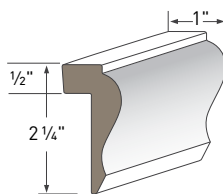
WAINSCOT CAP AZM-284 Length: 16'
