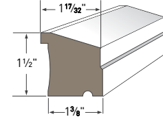
SUB SILL NOSE AZM-6933 Length: 16'
