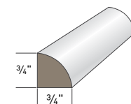
QUARTER ROUND AZM-105 Length: 16'
