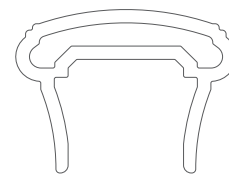
TRADEMARK RAIL™ TOP RAIL SIZE: 3.5" X 2.6" ONLY AVAILABLE IN WHITE
