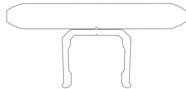
CONTEMPORARY RAIL TOP RAIL SIZE: 6.4" X 3" ONLY AVAILABLE IN CLASSIC BLACK & TRADITIONAL WALNUT
