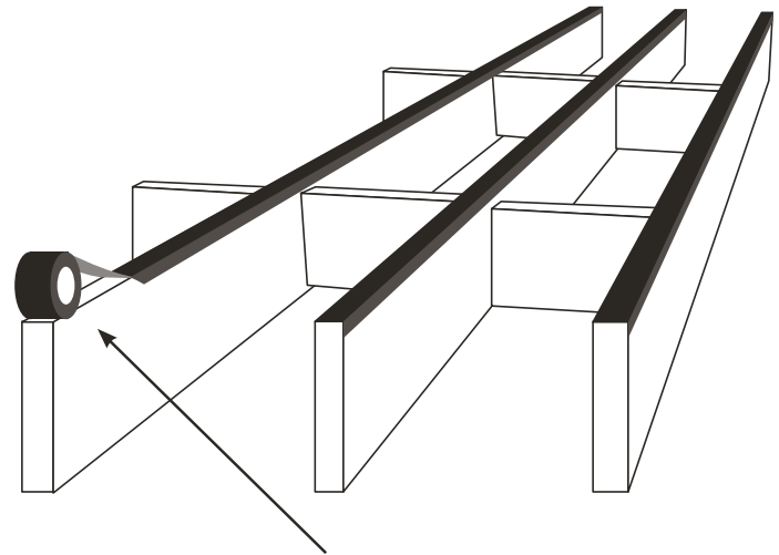
Apply PRO-Tac tape to the top of joists before installing deck boards.
