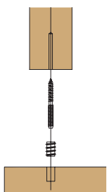
LJ-3004-3.5 Hanger Bolt & Threaded Insert
