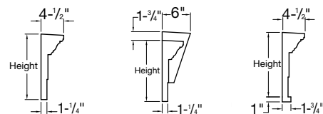
Standard w/ Keystone K9M w/ Bottom Trim*
