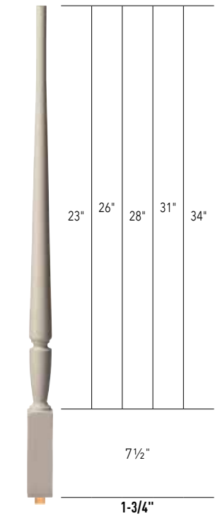
S2015 31" 34" 36" 39" 42"
