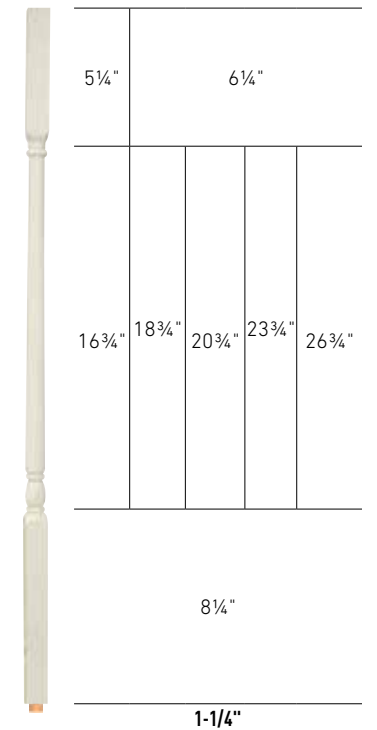
S5141 31" 34" 36" 39" 42"
