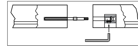
3001SP 2 3001 SP ZIPBOLT™ — 2-Pack
