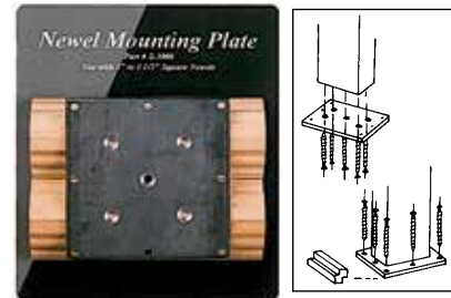
3006 NEWEL MOUNTING KIT W/PLATE 3006 PL PLATE ONLY
