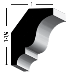
68 9/16 x 1-5/8 PRIMED 8' | 12'
