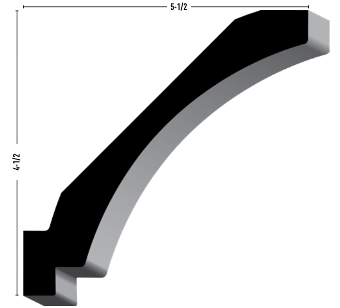
730 1-3/16 x 7 MDF 16'
