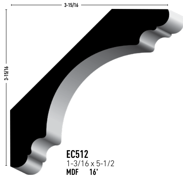
530 1-3/16 x 5-1/2 MDF 16'
