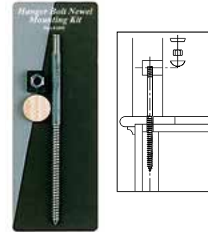
3008-10 NEWEL POST FASTENER 10-3/4"
