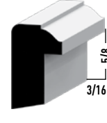
281 Back Band 11/16 x 1-1/8 PRIMED 16' PINE 8'
