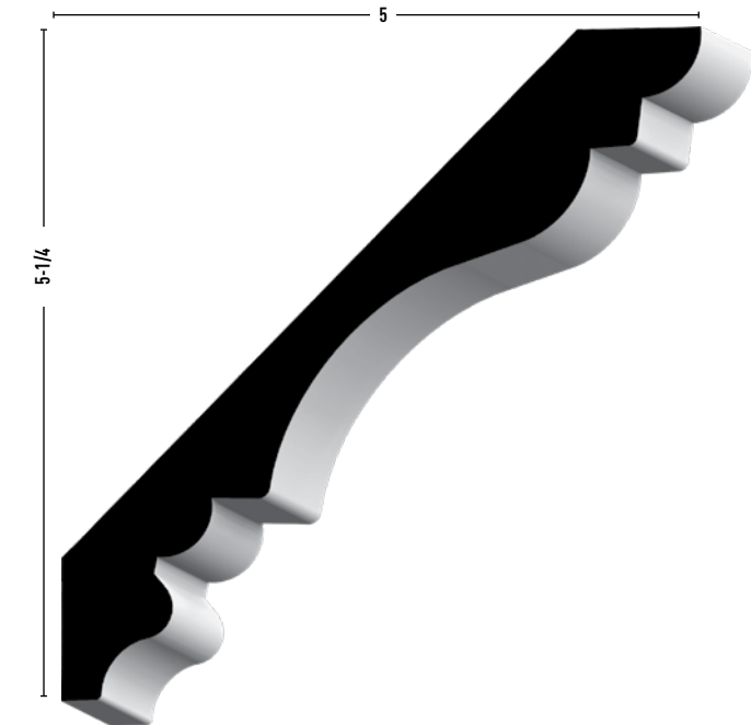
721 1 x 7-1/4 MDF 16'
