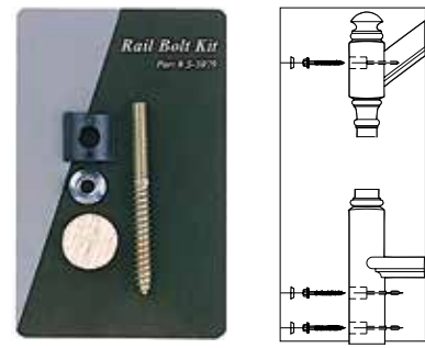
3001 / 3079 RAIL BOLT
