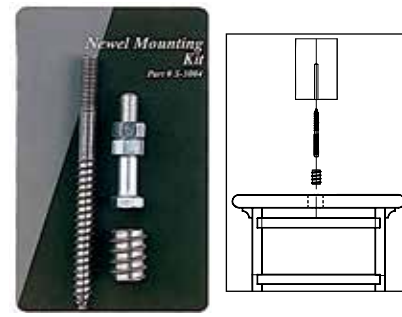
3004 NEWEL MOUNTING KIT
