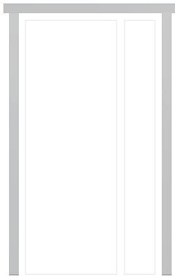
TDS-FLTFLT-4S4H Smooth Flat Trim Option A | 4" Side | 4" Header
